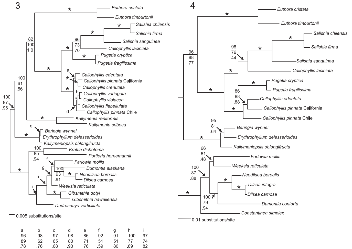
Figs 3, 4. Inclusion of the newly-determined species groups in phylogenetic analyses of representative Kallymeniaceae. Fig. 3. Phylogram inferred by Bayesian analyses of LSU data (letters denote support values listed below phylogram). Fig. 4. Phylogram inferred from a combined data set including LSU and COI-5P. Support values are listed for both phylogenies as Bayesian posterior probabilities and bootstrap and aLRT values for maximum likelihood analyses, respectively. Asterisks denote nodes that are strongly supported (posterior probability = 100%, bootstrap \geq 95% and aLRT values \geq 0.95) in all analyses.
